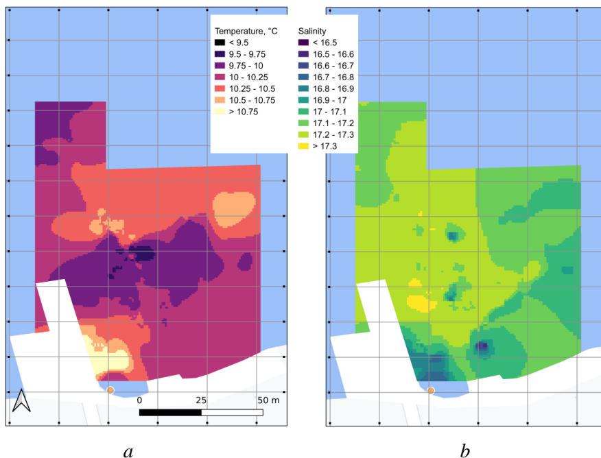
Fig. 4. Two-dimensional temperature (a) and salinity (b) field based on the in situ measurements performed by the TMA-21 sensor from aboard the USV near the rainwater discharge outlet in the Apollonova Bay on 02.04.2021. The result of IDW interpolation made using QGIS and Google Terrain basemap. Location of the rainwater discharge outlet is shown by an orange dot. Grid lines are drawn with the 20 m interval
