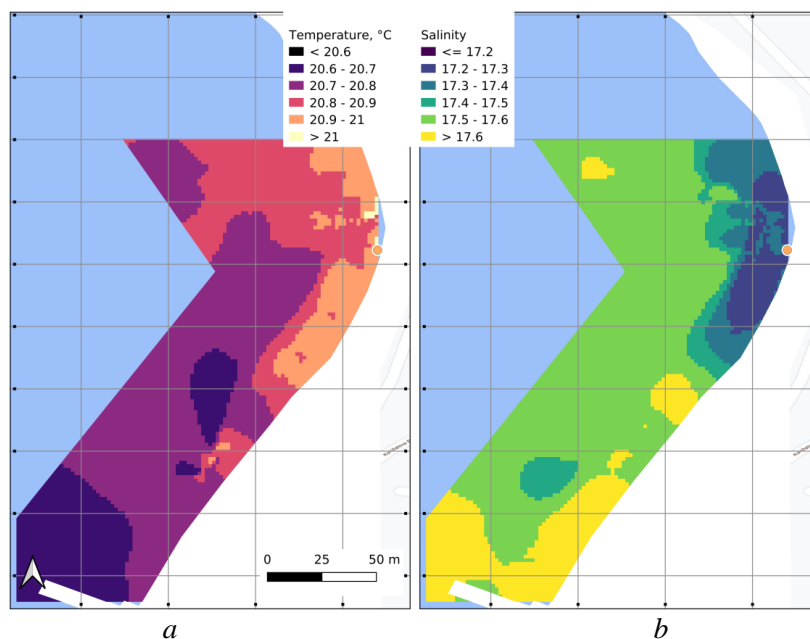
Fig. 5. Two-dimensional temperature ( a ) and salinity ( b ) field based on the in situ measurements performed by TMA-21 sensor from the board the USV near the rainwater discharge outlet in the Gollandiya Bay on 18.06.2021. The result of IDW interpolation made using QGIS and Google Terrain basemap. Location of the rainwater discharge outlet is shown by an orange dot. Grid lines are drawn with the 40 m interval
