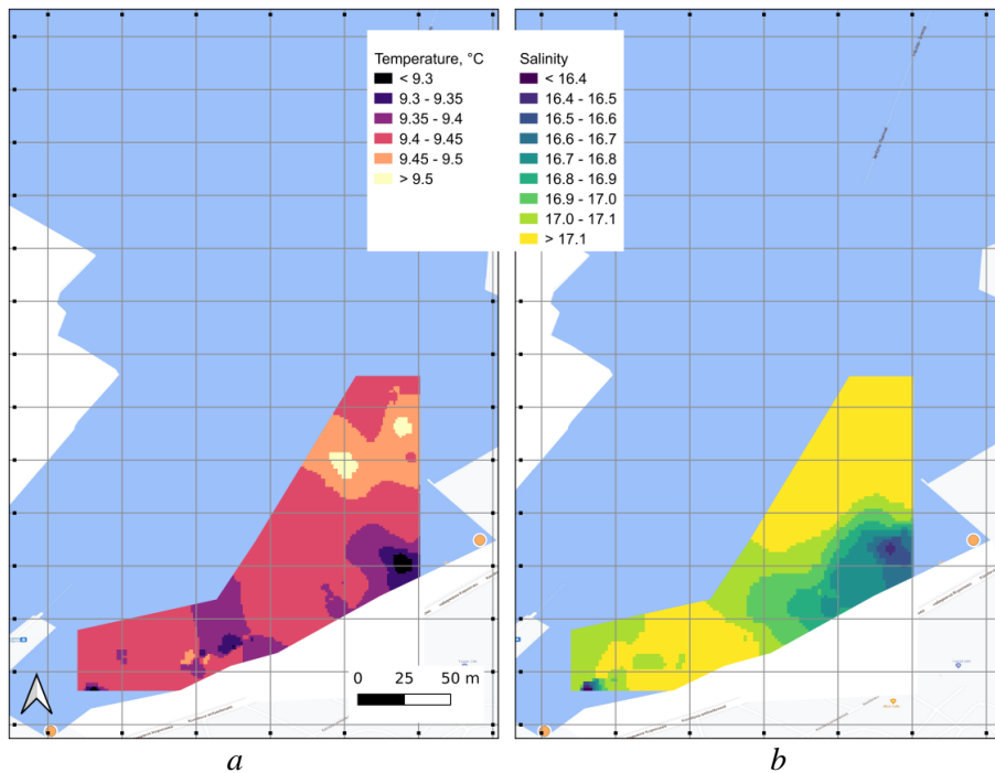
Fig. 6. Two-dimensional temperature ( a ) and salinity ( b ) field based on the in situ measurements performed by TMA-21 sensor from the USV board near the rainwater discharge outlet in the Artilleriyskaya Bay on 08.04.2021. The result of IDW interpolation made using QGIS and Google Terrain basemap. The location of the rainwater discharge outlet is shown by an orange dot. Grid lines are drawn with the 40 m interval
